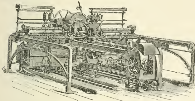
THE SELF-ACTING MULE.
